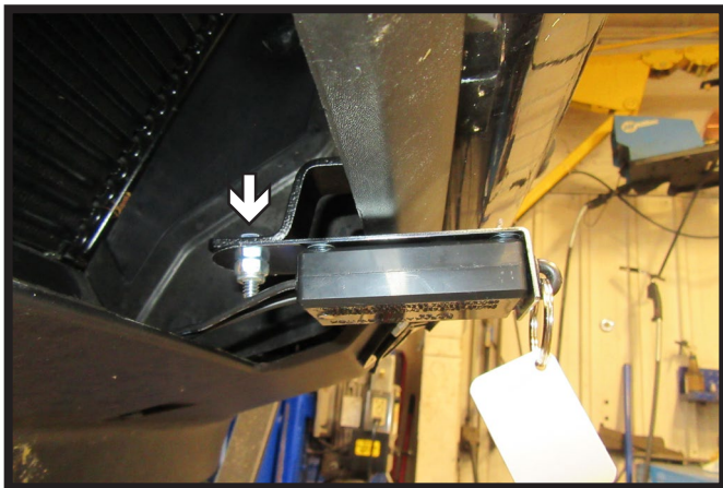
8c. Optional Breakaway: Attach breakaway switch to the breakaway bracket using the provided hardware.
