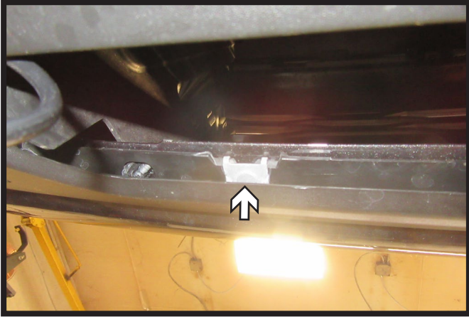
8a. Optional Breakaway: Using a 10MM socket, remove the nut from the gray clip in the fascia opening.
