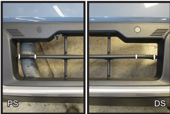
27. Using a reciprocating saw, remove the horizontal slats on each side of the vehicle between the white marks as shown to allow room for the removable tabs.
