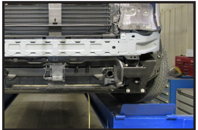
28. Reinstall the black box on the driver side of the vehicle. Reattach the wire loom to front of the box and to the bottom bolt on the backside. If the box touches the baseplate bolt head, bend back plate slightly to create clearance.
