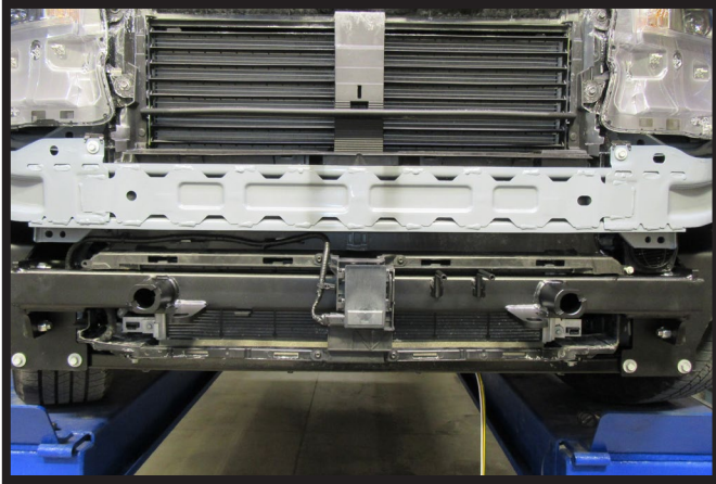
25. Reinstall the ACC mounting bracket.
