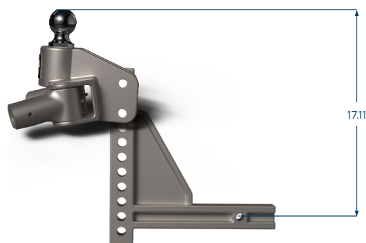
11-Hole Receiver, 1-1/4" Adjustment Increments
