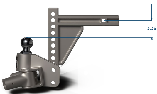
11-Hole Receiver, 1-1/4" Adjustment Increments
