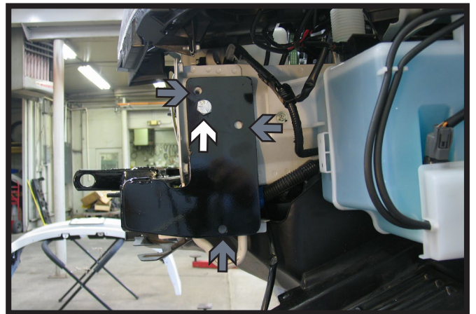
8. Slide the baseplate onto the vehicle lining up the existing hole in the frame with the baseplate (white). Install a 1/2"-13 x 1-1/4" bolt into the hole with 1/2" flat washer, lock washer and nut on the inside of the frame. Do this on both sides of the vehicle. Level the baseplate and fully tighten the 1/2" hardware. Using a 13/32" drill bit, drill the remaining six (6) holes of the baseplate thru the frame (gray). There are three (3) on each side.
