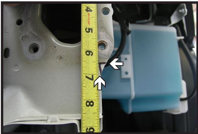
7. Using a reciprocating saw, make a notch down 6-1/2" from the top of the frame and flush with the outside of the frame as shown. Do this on both sides of the vehicle.
