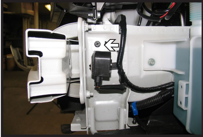
5. Using a 10MM socket, remove the screw from the sensor on the driver side.
