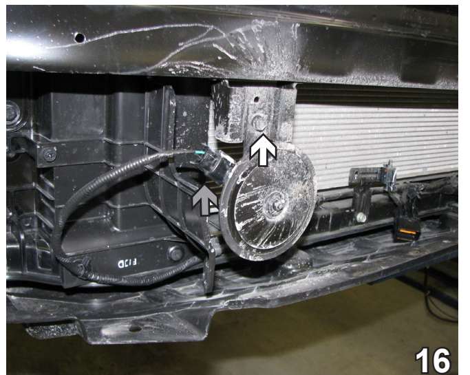
16. Using the 10MM socket, remove the bolt attaching the horn to the bracket (white arrow). Unplug the horn (gray arrow).
